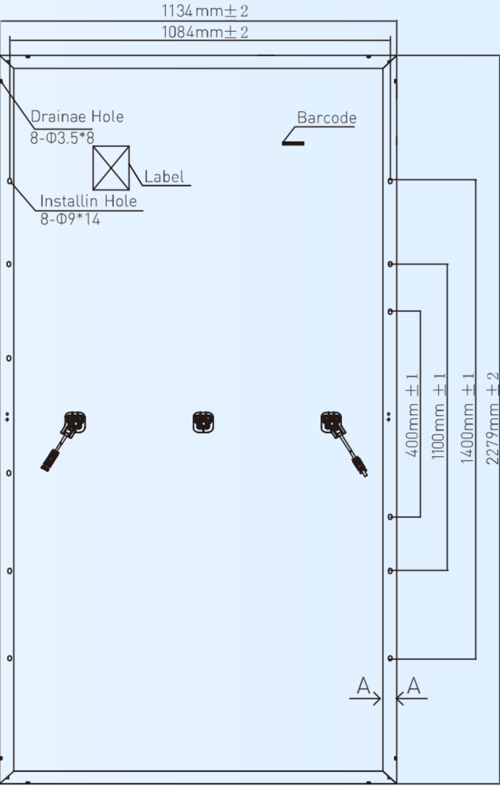
Back View
